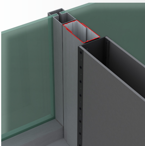
WALL-TO-MULLION
